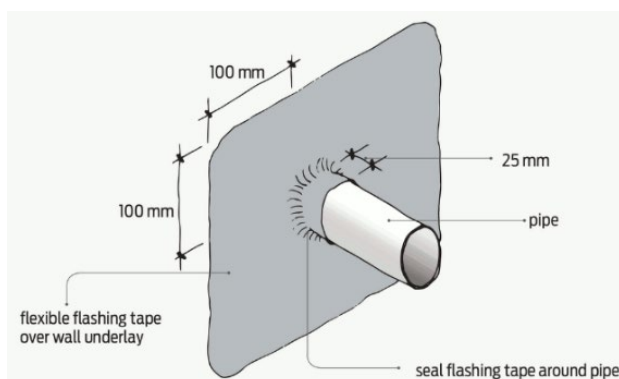
DIAGRAM 8 – service penetrations
