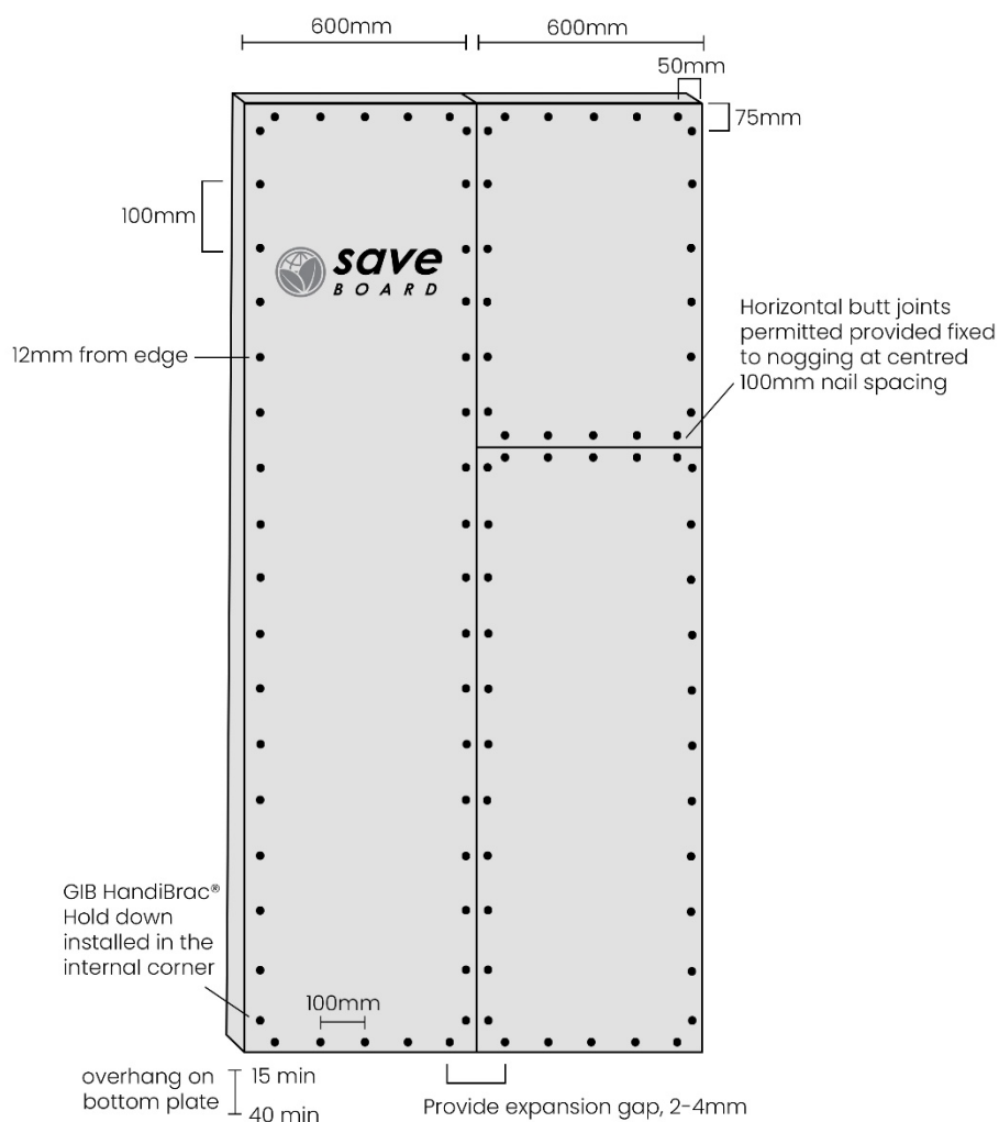
DIAGRAM 5 – System 2 saveBOARD betterBRACE 10mm – 600mm x 2400mm bracing element
