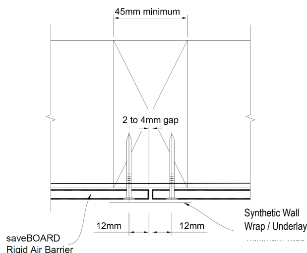
DIAGRAM 1 – Vertical Board Layout
