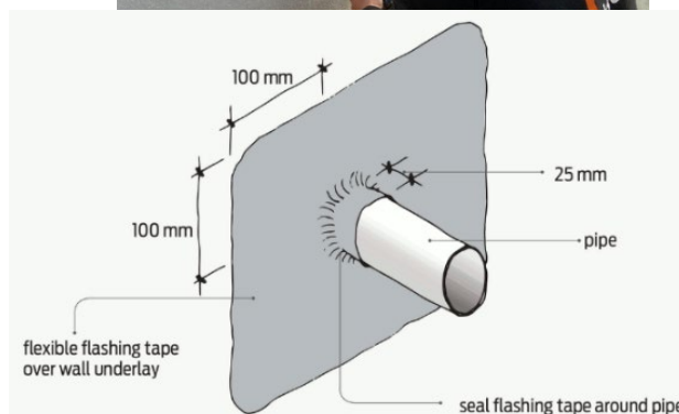
DIAGRAM 14 – service penetrations
